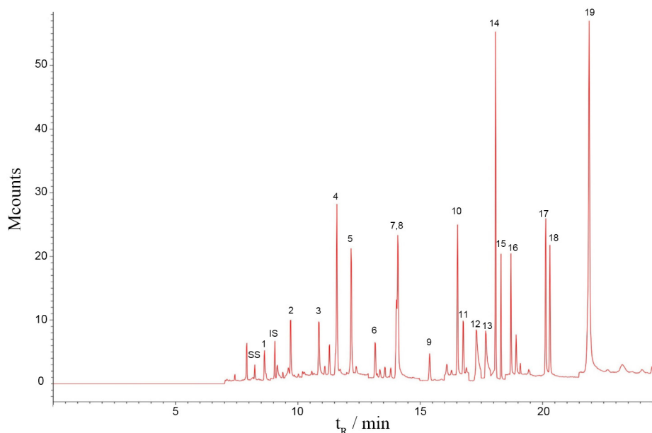
Figure 1. Gas chromatography with mass spectrometry (GC-MS) in the selected ion monitoring (SIM) total ion chromatogram of a blank matrix matched standard solution at 1.0 \text{ mg kg}^{-1} containing all the selected pesticides: (1) chlorothalonil, (2) metalaxil, (3) triadimefom, (4) cyprodinil, (5) procimidone, (6) endosulfan alpha, (7) miclobutanil, (8) buprofezin, (9) endosulfan beta, (10) trifloxystrobin, (11) endosulfan sulfate, (12) tebuconazol, (13) epoxiconazol, (14) bifenthrin, (15) fenpropathrin, (16) tetradifon, (17) cis -permethrin, (18) trans -permethrin, (19) etofemprox, (SS) quintozone and (IS) caffeine.
